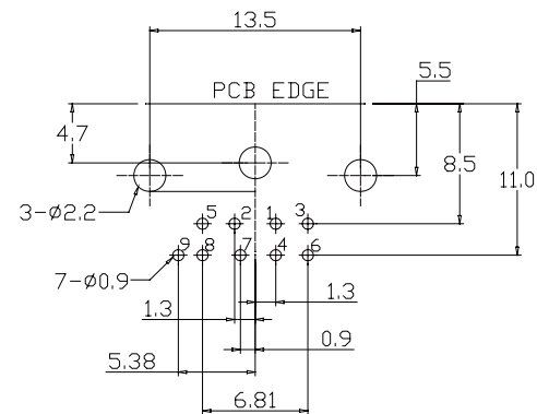
P.C.B. RECOMMEND LAYOUT BOTTOM VIEW
